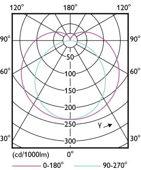
Light Distribution Diagram - MAS LEDtube HF 1500mm UO 24W865 T8
